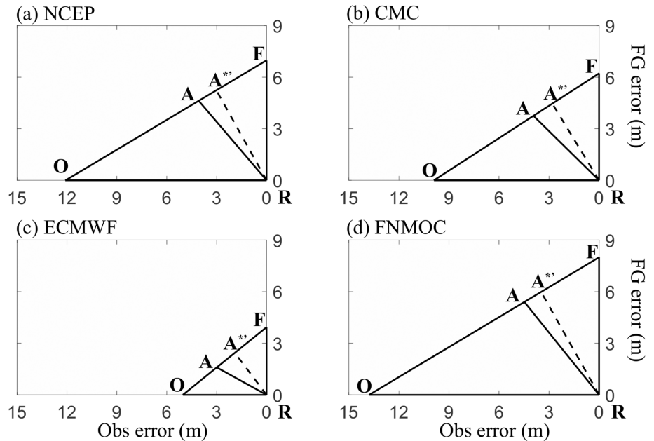
FIGURE 10 Same as the schematic in Figure 3, except based on parameters estimated from four operational DA systems: (a) NCEP, (b) CMC, (c) ECMWF, and (d) FNMOC. See text for further details.
