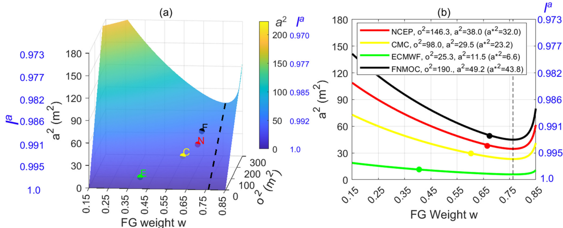
FIGURE 11 (a) Variation of a^2 as a function of w and a continuous (panel a) and discrete function of o^2 (b, for o^2 = 146.3, 98.0, 25.3 , and 190.0 \text{ m}^2 for the operational DA systems at NCEP (red, N), CMC (yellow, C), ECMWF (green, E), and FNMOC (black, F), respectively), with e^{\alpha \cdot \Delta t} = 1.31 . Values of a^2 for the four systems are marked by solid circles. Black dashed lines indicate the optimal analysis error variance a^{*2} .
