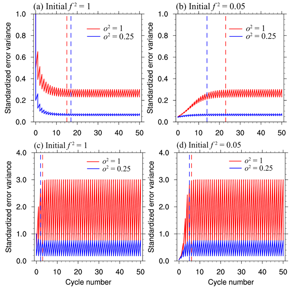
FIGURE A1 Variation of the standardized analysis ( a^{*2} ) and first-guess ( f^2 ) error variances with the number of the assimilation-forecast cycle given the initial first-guess error variance f^2 = 1 (a,c) and f^2 = 0.05 (b,d). The standardized observational error variance is o^2 = 1 (red solid line) and 0.25 (blue solid line), while the error growth rate e^{a \cdot \Delta t} is 1.31 (panels a,b) and 4 per six hours (panels c,d). For each experiment, the dashed vertical line indicates the number of cycles after which analysis error variance reaches 99.9% of its saturation value. [Colour figure can be viewed at wileyonlinelibrary.com ]
